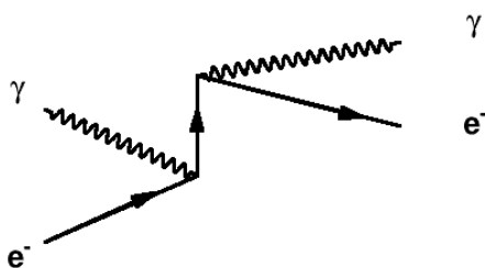
Figur 10.5: Feynman-diagram for Compton-spredning
